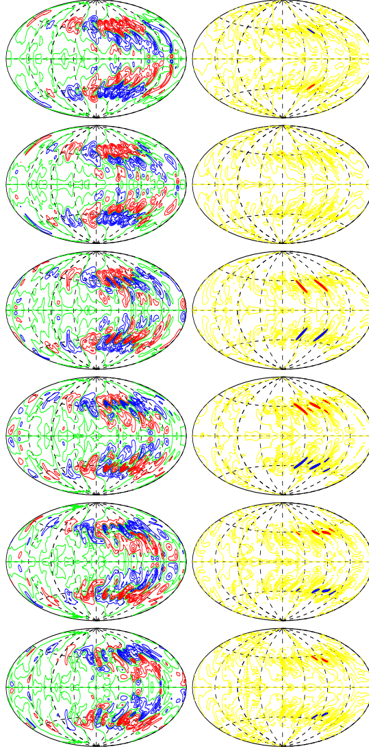
Figure 1: Half a period of oscillation in the case \eta = 0.65 , P = 1 , \tau = 2000 , R_e = 150000 , P_m = 4 , \beta = 1.5 with stress-free velocity boundary condition at r = r_o and no-slip at r = r_i . The left column shows contour lines of B_r at r = 1 and the right column shows contour lines of -\frac{\partial g}{\partial \theta} at r = 0.9 . The time interval between the snapshots is 0.0112.
