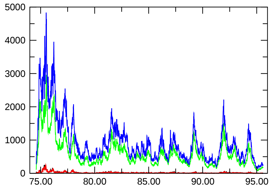
E_{\text{magn,dip.}}
