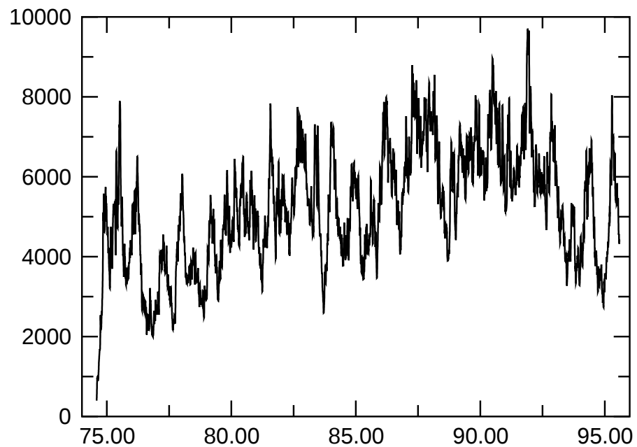
e065p1t2r150000m1p6mvbcFDsolrot1 E_{\text{magn}}
