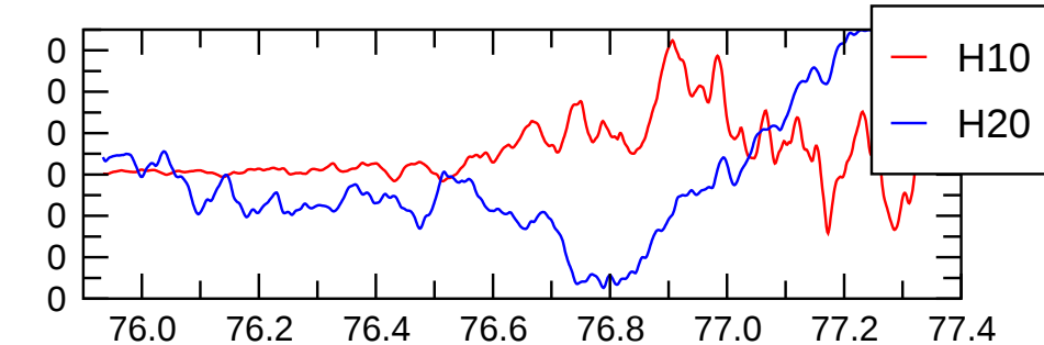
H10, H20 at r=r_i+1 , (magn)
