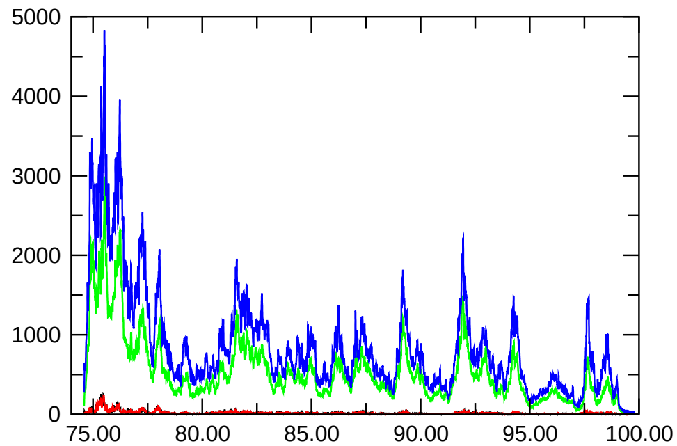
E_{\text{magn,dip.}}
