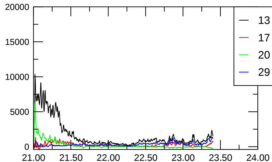
fluct-tor
