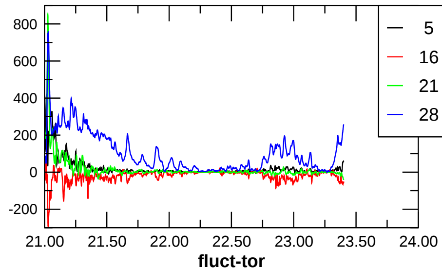
mean-tor
