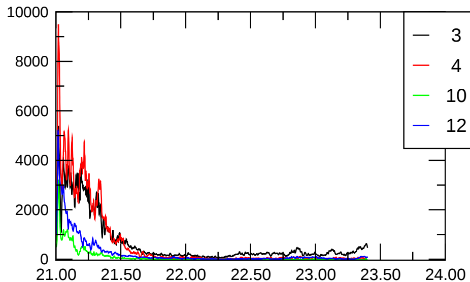
fluct-pol
