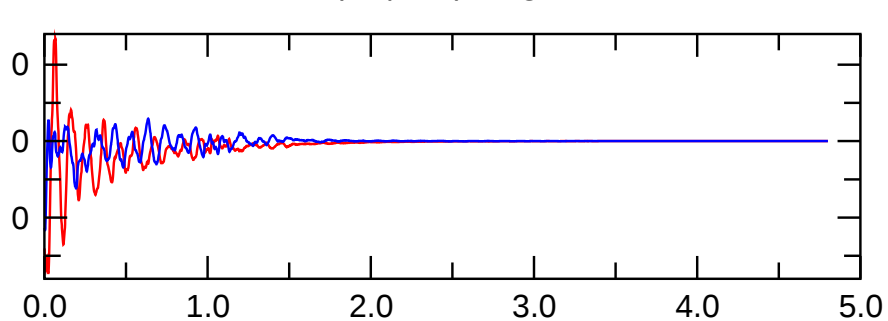
\text{pol}(m=0) magn.
