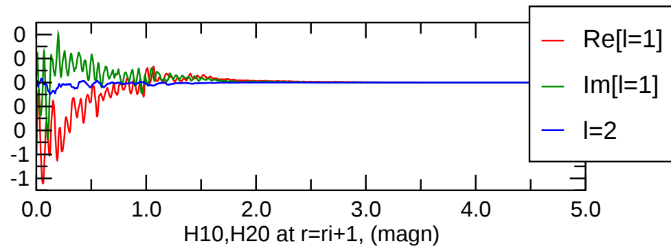
\text{pol}(m=1) magn.
