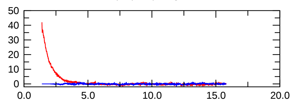
\text{pol}(m=0) magn.
