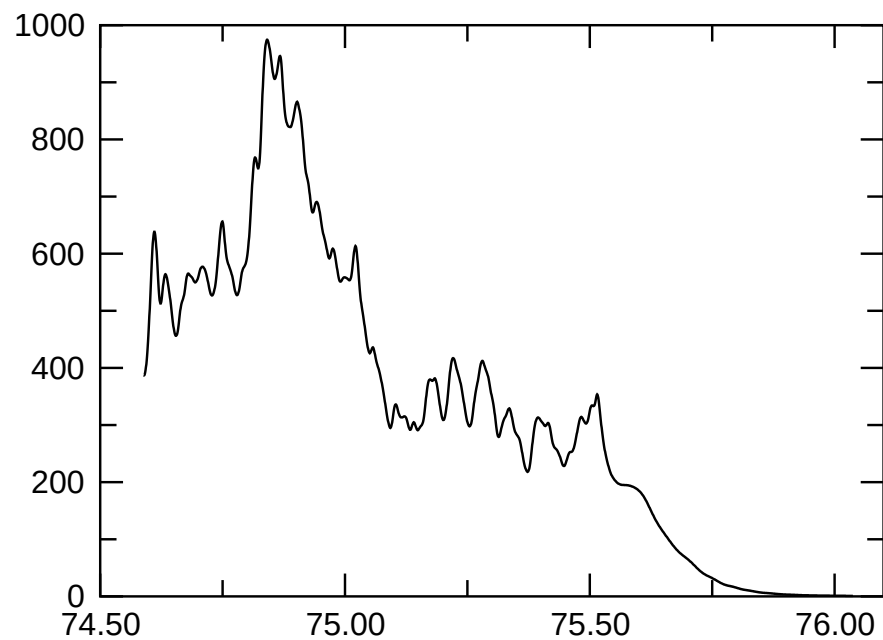
e065p1t4r170000m1p4mvbcFDsolrot1.5 E_{\text{magn}}
