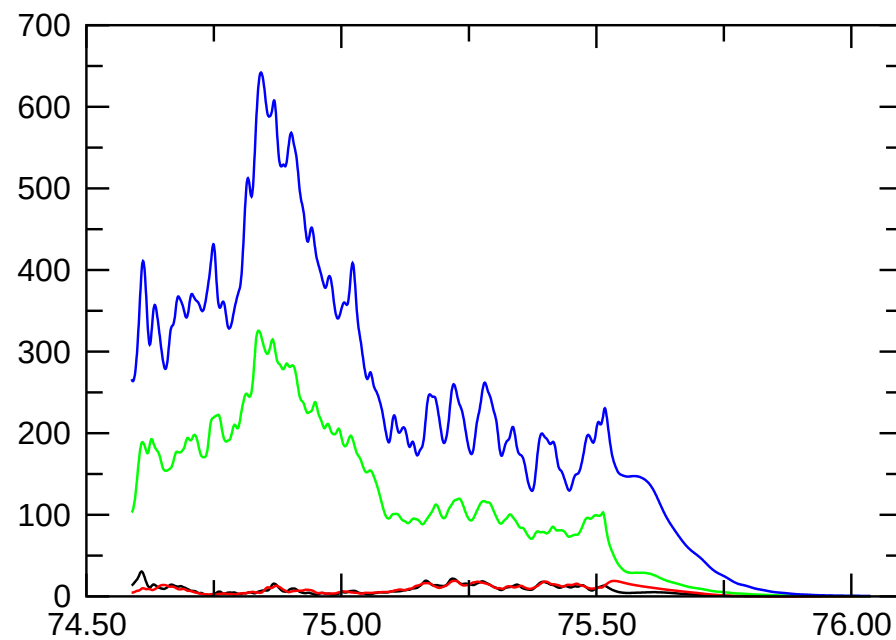
E_{\text{magn,dip.}}
