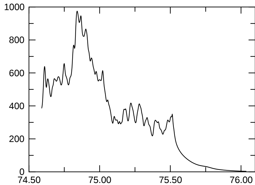
e065p1t6r170000m1p4mvbcFDsolrot1.5 E_{\text{magn}}
