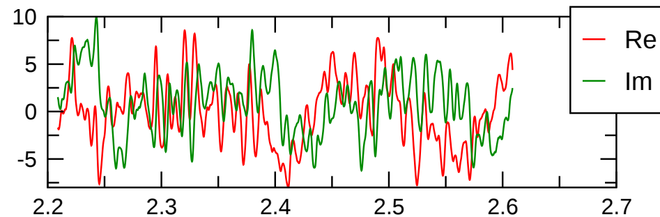
tor(m=0) magn.
