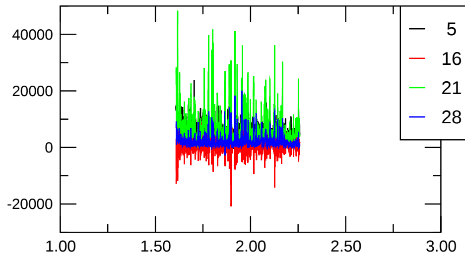
fluct-tor
