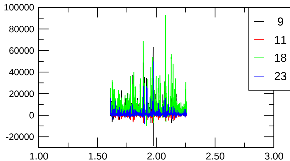
fluct-pol
