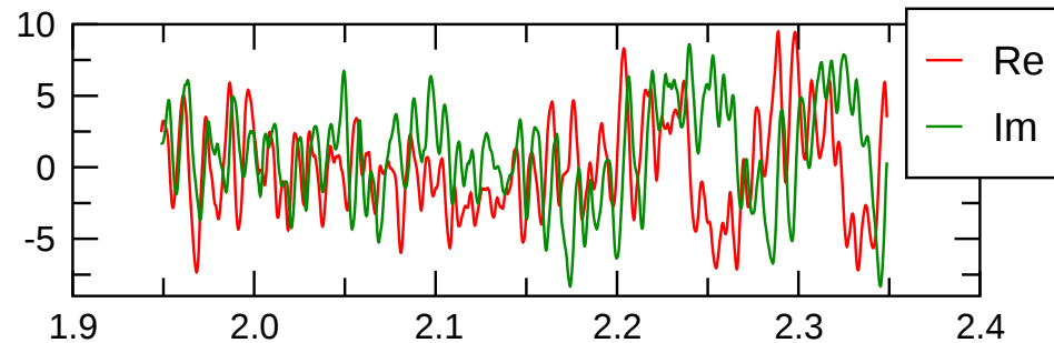
tor(m=0) magn.
