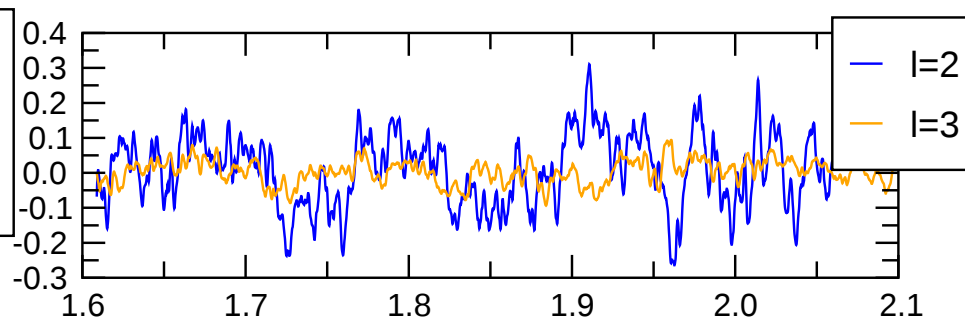
\text{pol}(m=0) magn.
