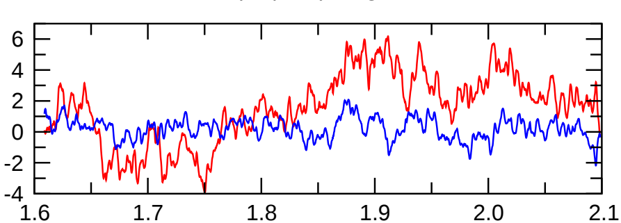
\text{pol}(m=0) magn.
