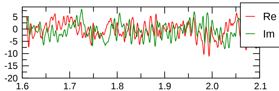
\text{tor}(m=0) magn.
