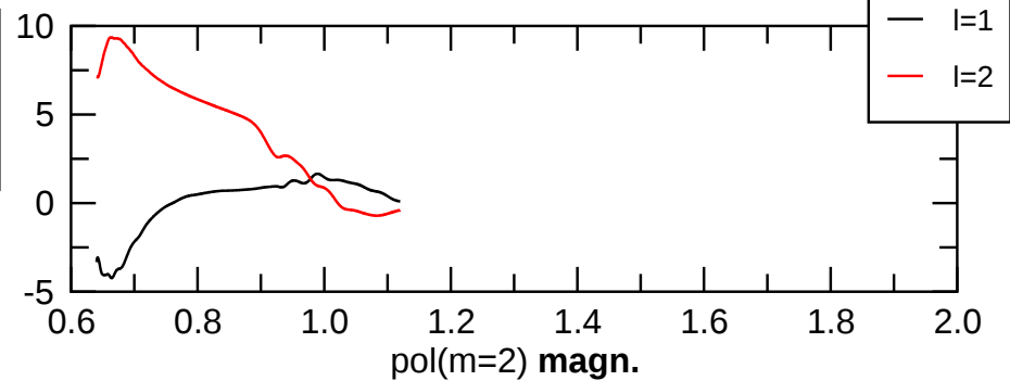
tor(m=0) magn.
