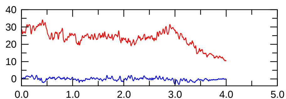
\text{pol}(m=0) magn.
