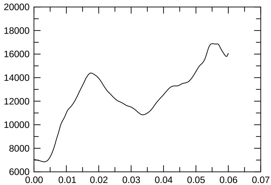
e06p09t2re500000m1p3mvbc E_{\text{magn}}
