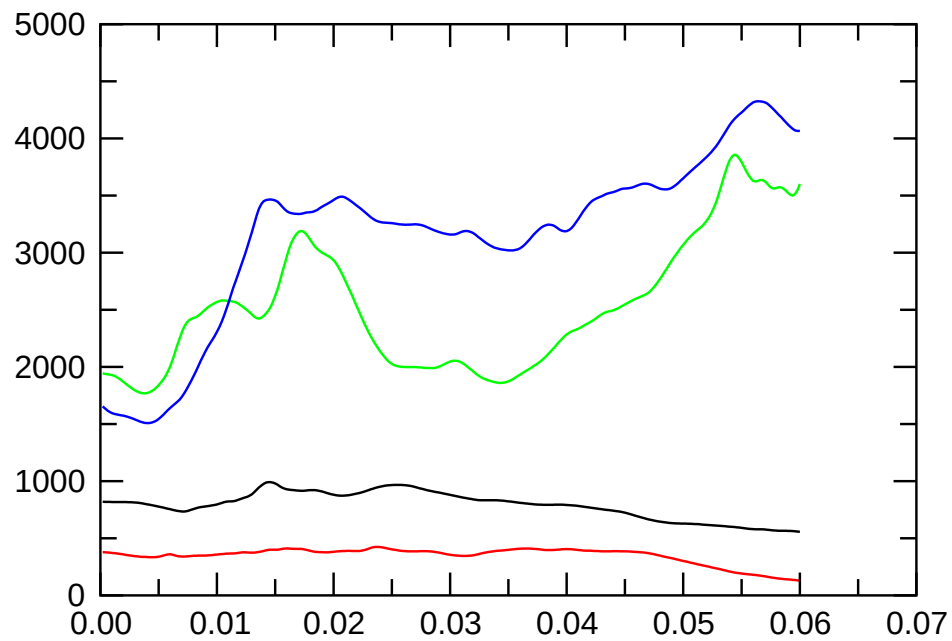
E_{\text{magn,dip.}}
