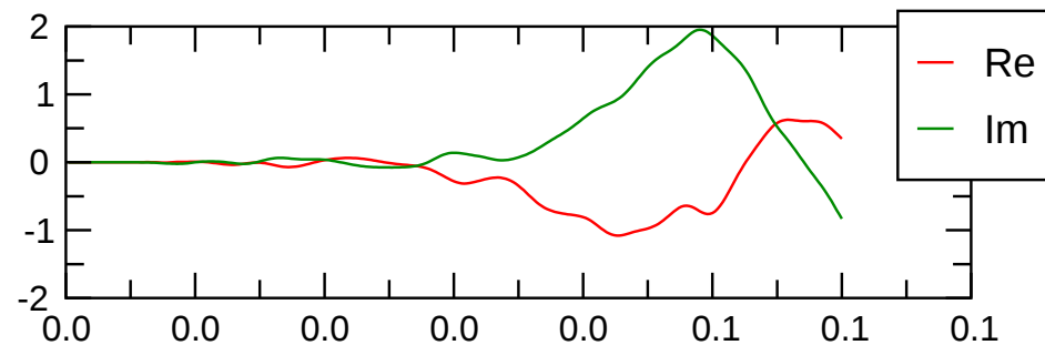
tor(m=0) magn.
