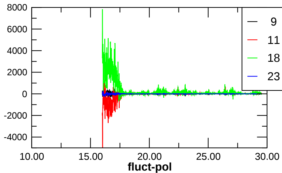
mean-pol
