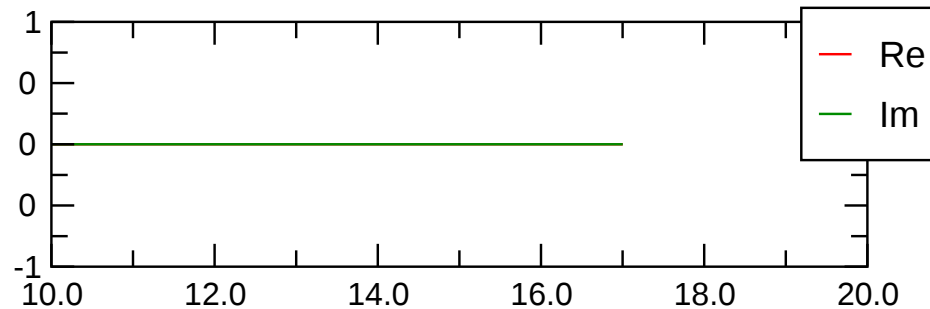
tor(m=0) magn.
