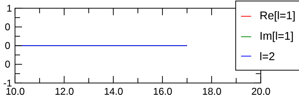
H10,H20 at r=ri+1, (magn)
