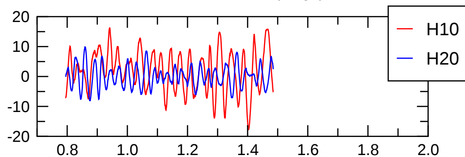
H10, H20 at r=r_i+1 , (magn)
