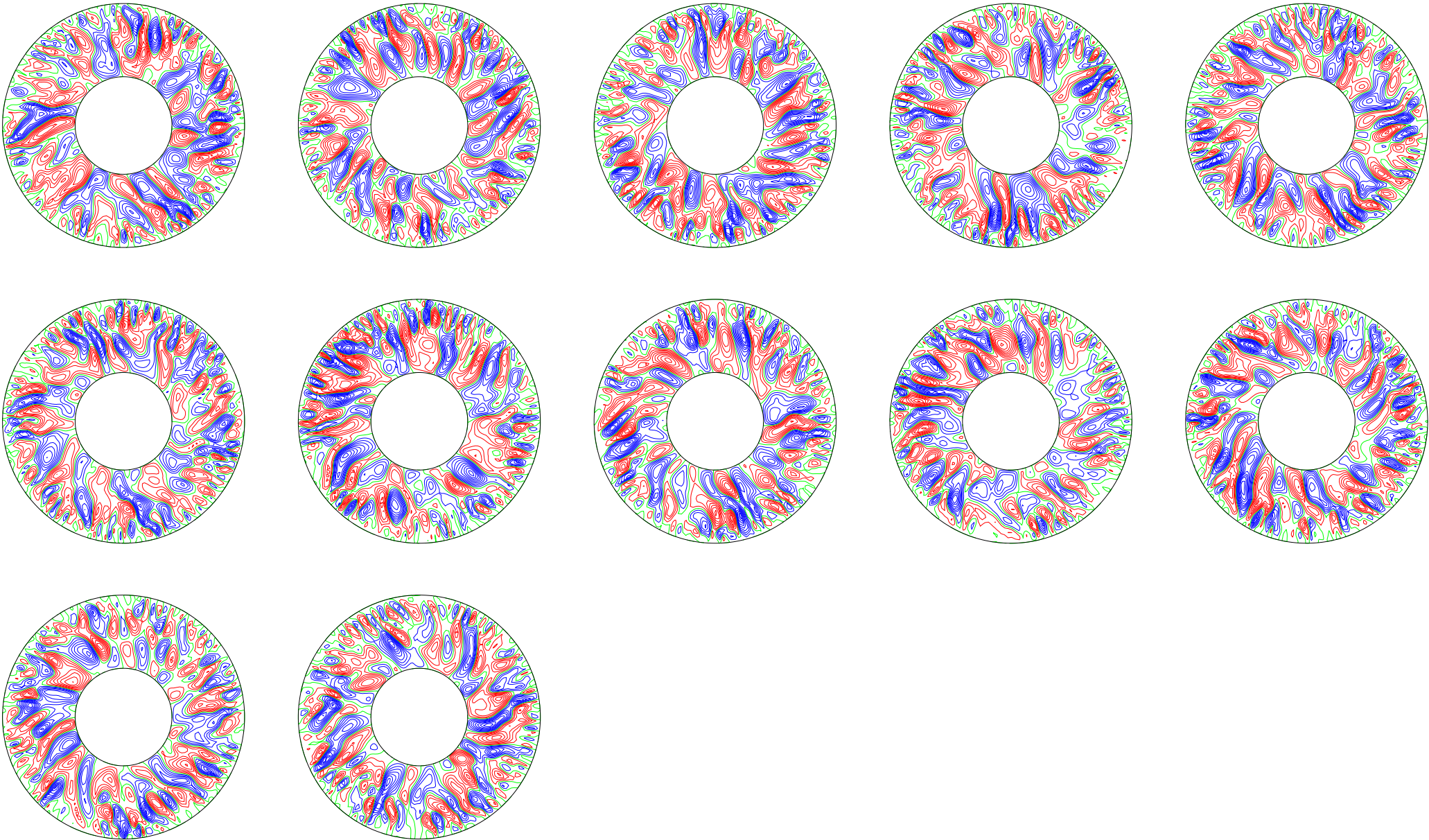
poloidal streamlines, (t[i] dt[i] t[i+1]): 12.51717 ( 0.035 ) 12.90228
