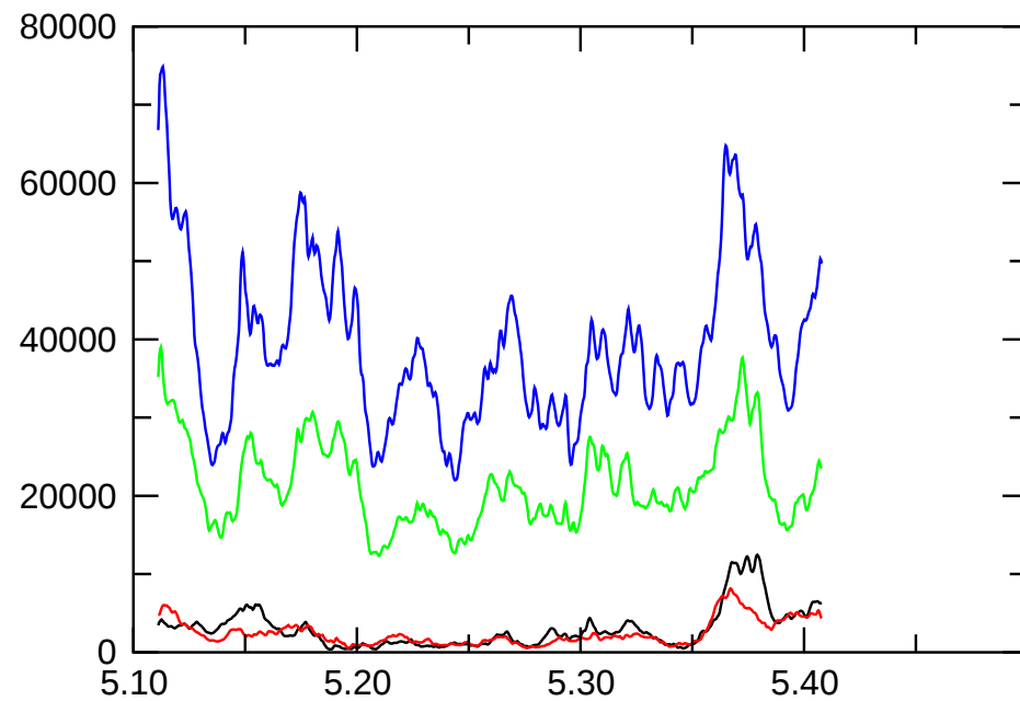
E_{\text{magn,dip.}}
