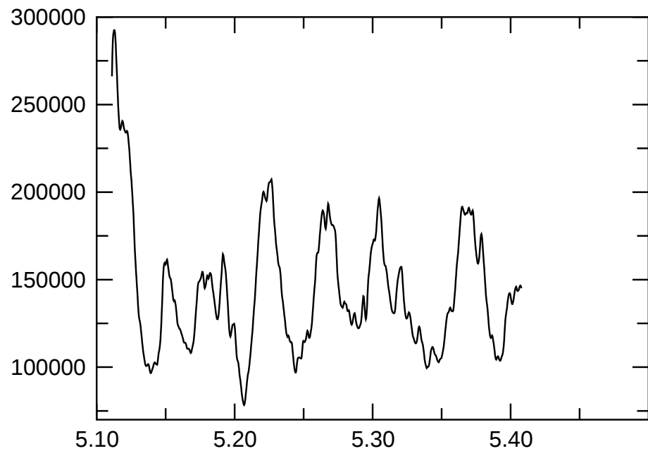
p065t30r3500000m1p1.3FROMp05pm1 E_{\text{magn}}
