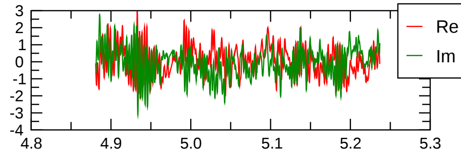
tor(m=0) magn.
