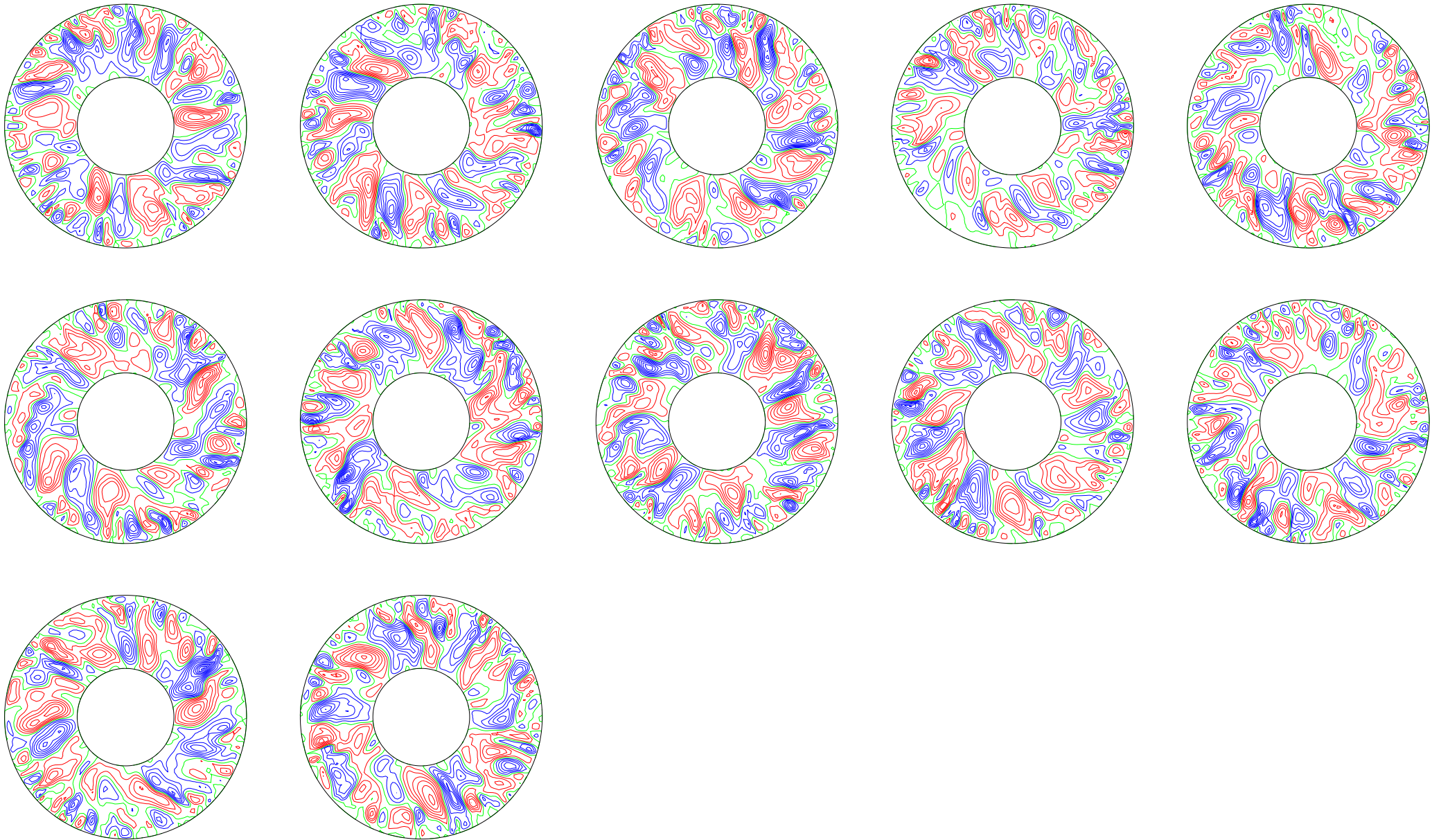
poloidal streamlines, (t[i] dt[i] t[i+1]): 5.09684 ( 0.004 ) 5.140851
