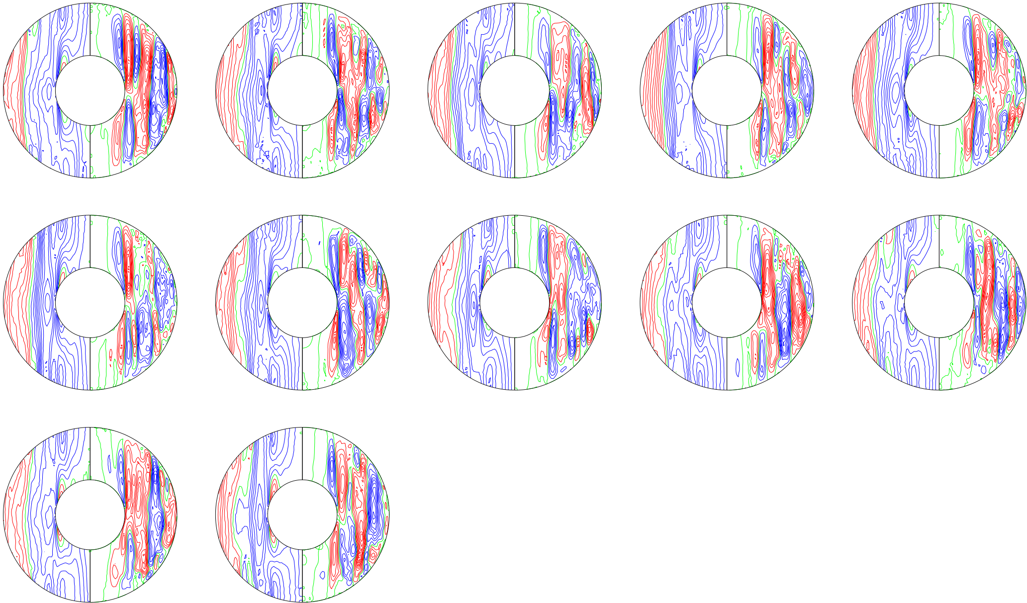
Uphi & merid strlines (merid. cut), (t[i] dt[i] t[i+1]): 5.048828 ( 0.004 ) 5.092839
