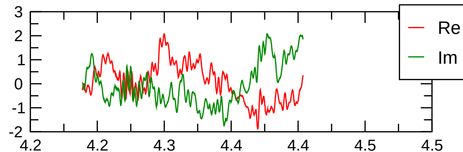
tor(m=0) magn.
