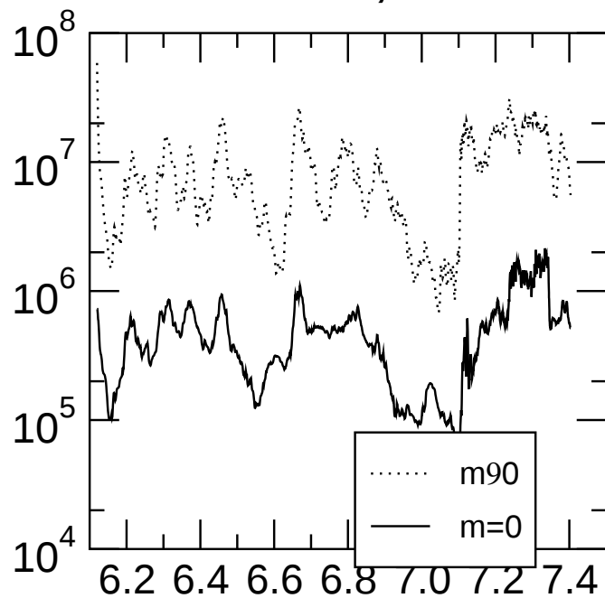
ohmic diss., toroidal
