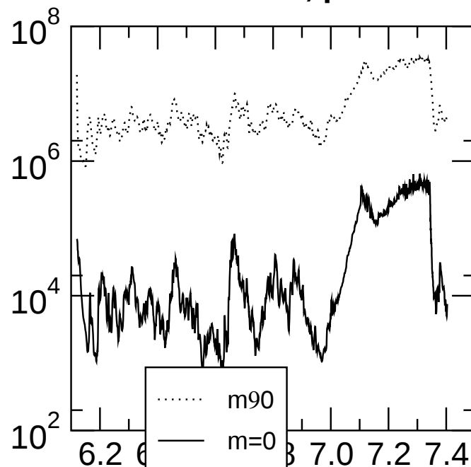
viscous diss., poloidal
