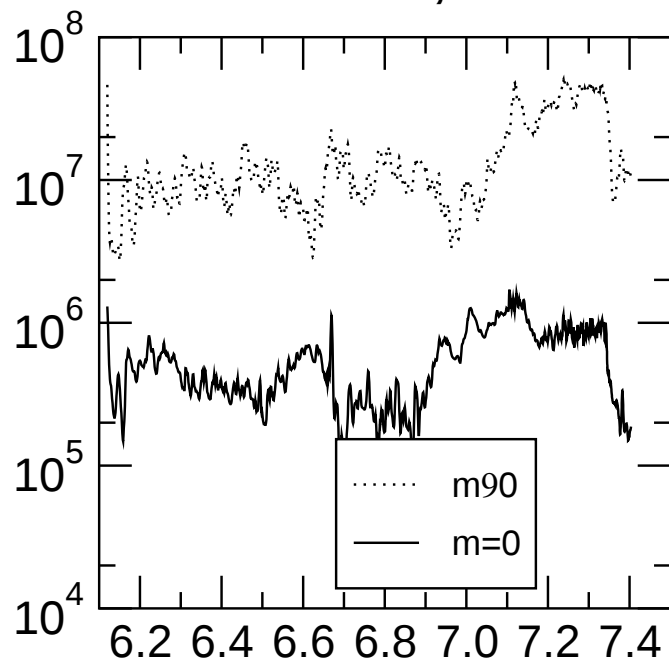
viscous diss., toroidal
