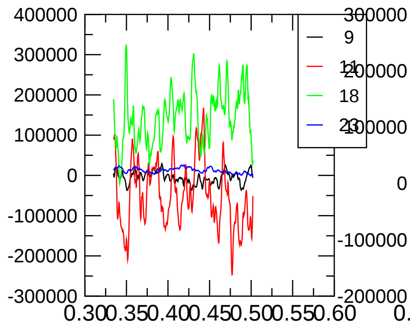
fluct-pol
