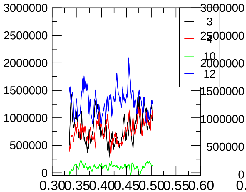
fluct-pol
