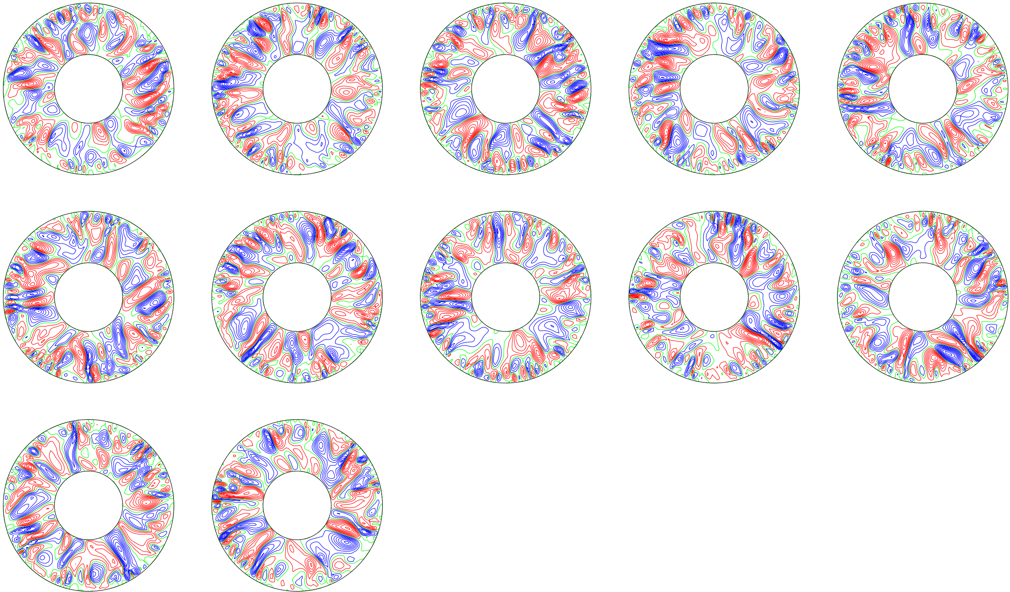
poloidal streamlines, (t[i] dt[i] t[i+1]): 3.48858 ( 0.01 ) 3.598591
