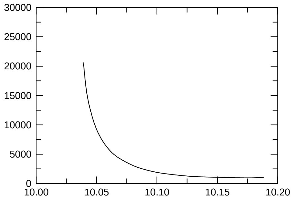
p2t50r3500000m1p4UP E_{\text{magn}}
