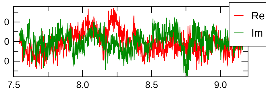
tor(m=0) magn.
