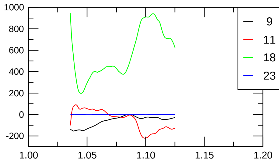
fluct-pol
