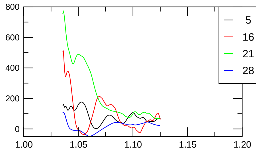
fluct-tor
