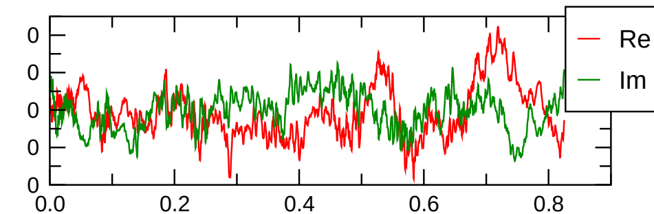
tor(m=0) magn.
