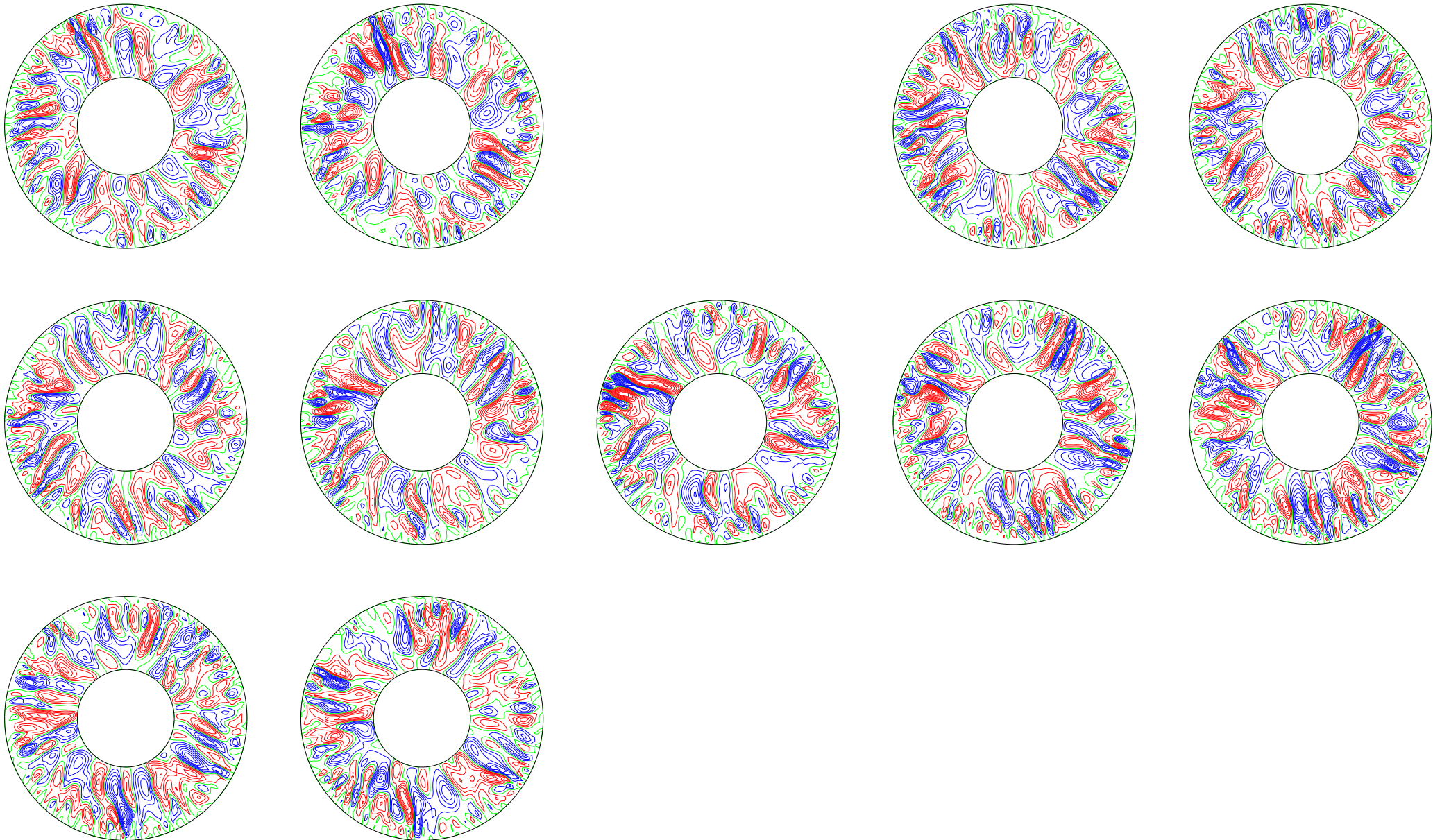
poloidal streamlines, (t[i] dt[i] t[i+1]): 0.065013 ( 0.005 ) 0.120024
