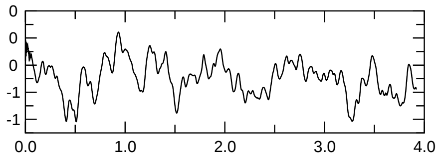
Btor(l=2,m=2) magn.
